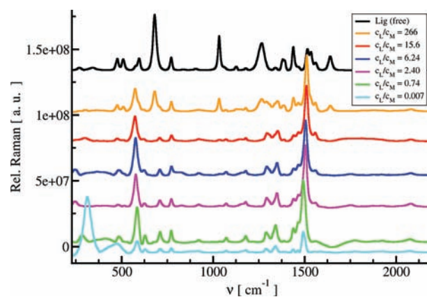
Figure 4. Titration of deferiprone with ferric chloride solution monitored by Raman spectroscopy. For the concentration ratio of 266, the intensities of free ligand ( 680\text{ cm}^{-1} ) and the 1:3 complex ( 573\text{ cm}^{-1} ) are almost equal. This approximately corresponds to 263 times enhancement of the Raman signal. The red spectrum (red lines) was selected as the best signal corresponding to the M:L 1:3 complex. The main bands maintained their positions while the ligand bands completely disappeared because of their relatively weak intensity in the preresonance.
