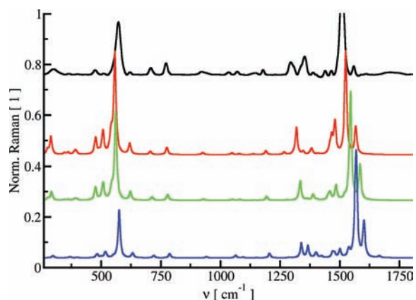
Figure 6. Experimental (black lines) and DFT/6-311++G**/CPCM (B3LYP, red lines; B3PW91, green lines; CAM-B3LYP, blue lines, Boltzmann-averaged) deferiprone complex Raman spectra.
