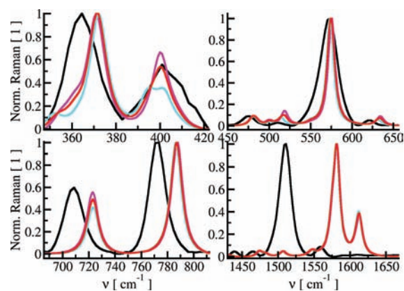
Figure 9. Experimental (black line) and CAM-B3LYP/MDF10 (Fe); 6-31+G** (other atoms)/CPCM calculated spectra in selected regions. A isomer (magenta lines), B isomer (cyan lines), Boltzmann average (red lines).
